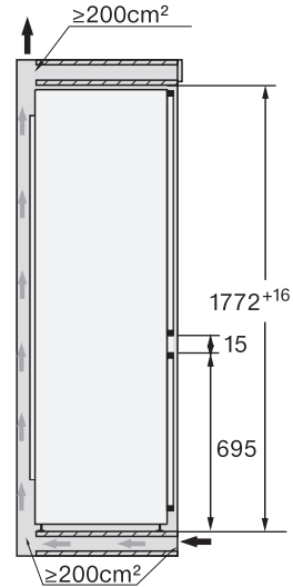
KFN 7734 F, KFN 7734 D, KFN 7744 E, KFN 7764 D, KFN 7785 D
